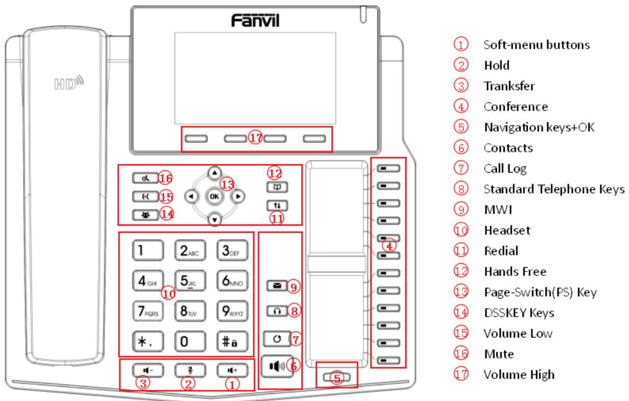
Figure 3 - Keypad
